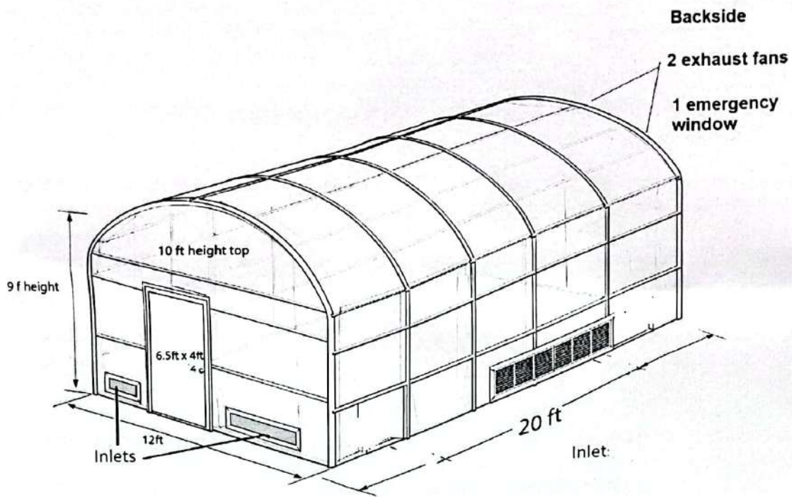
Solar Dehydration Unit
